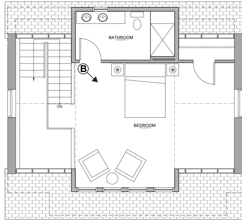
2ND FLOOR
