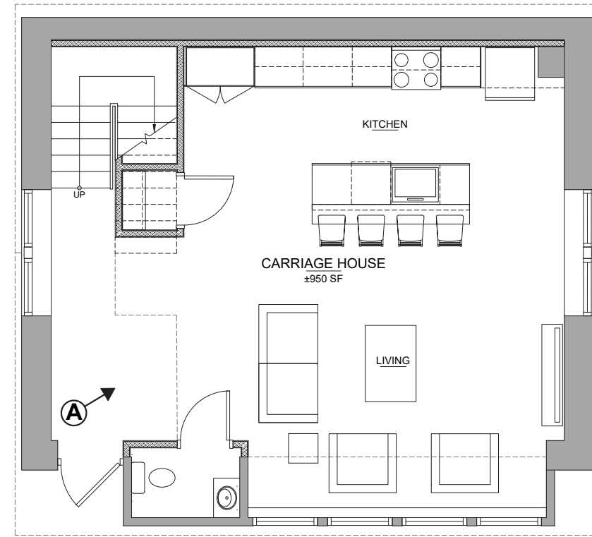
1ST FLOOR
